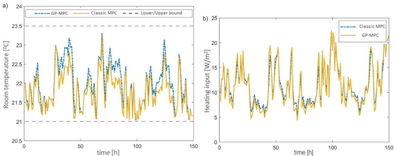
Figure 5. The closed-loop performances of classic MPC and GPs-based MPC law: a) room temperature, b) heating input
