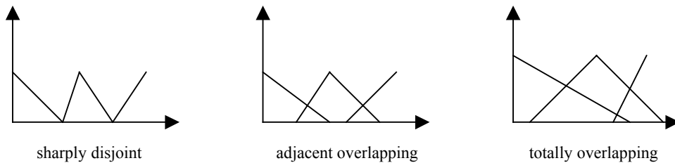
Fig. 3. Three kinds of fuzzy classification
