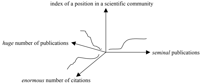
Fig. 2. Granulands determining the class of scientists
